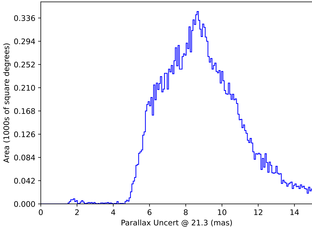
ddf_acor_sf10_lsf20_lsr50_v3.4_10yrs All sky y band only: Parallax Uncert @ 21.3
