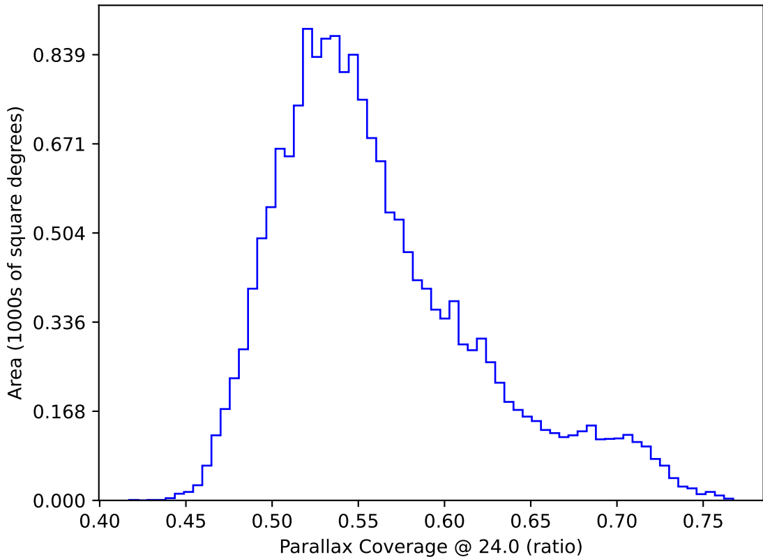
ddf_acor_sf10_lsf20_lsr50_v3.4_10yrs WFD: Parallax Coverage @ 24.0
