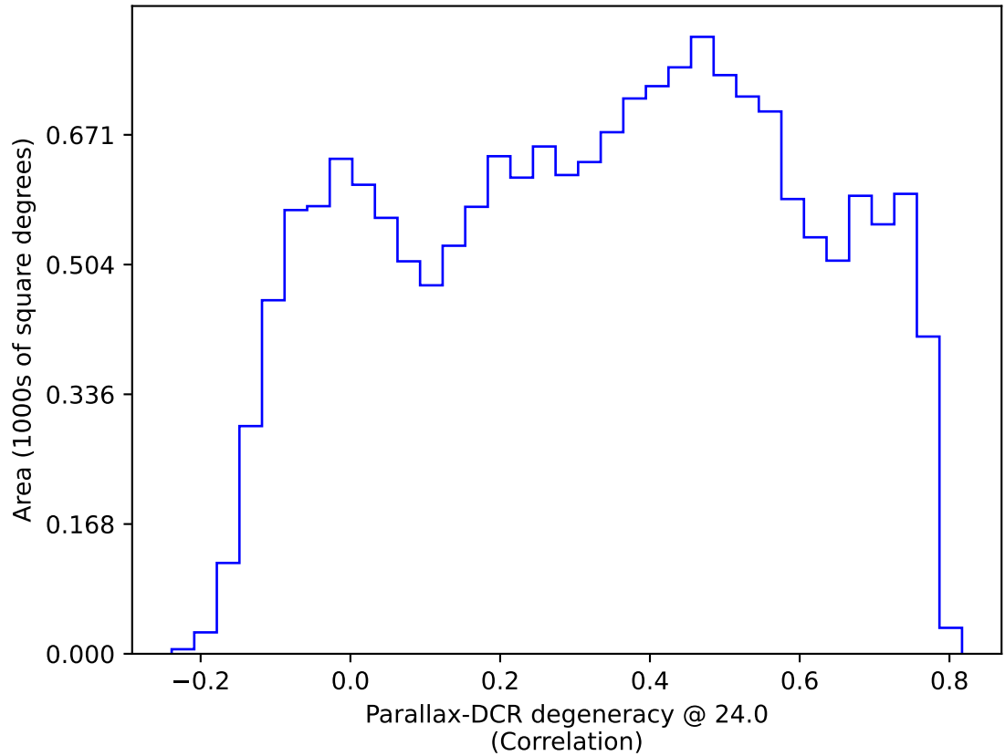
ddf_acor_sf10_lsf20_lsr50_v3.4_10yrs WFD: Parallax-DCR degeneracy @ 24.0
