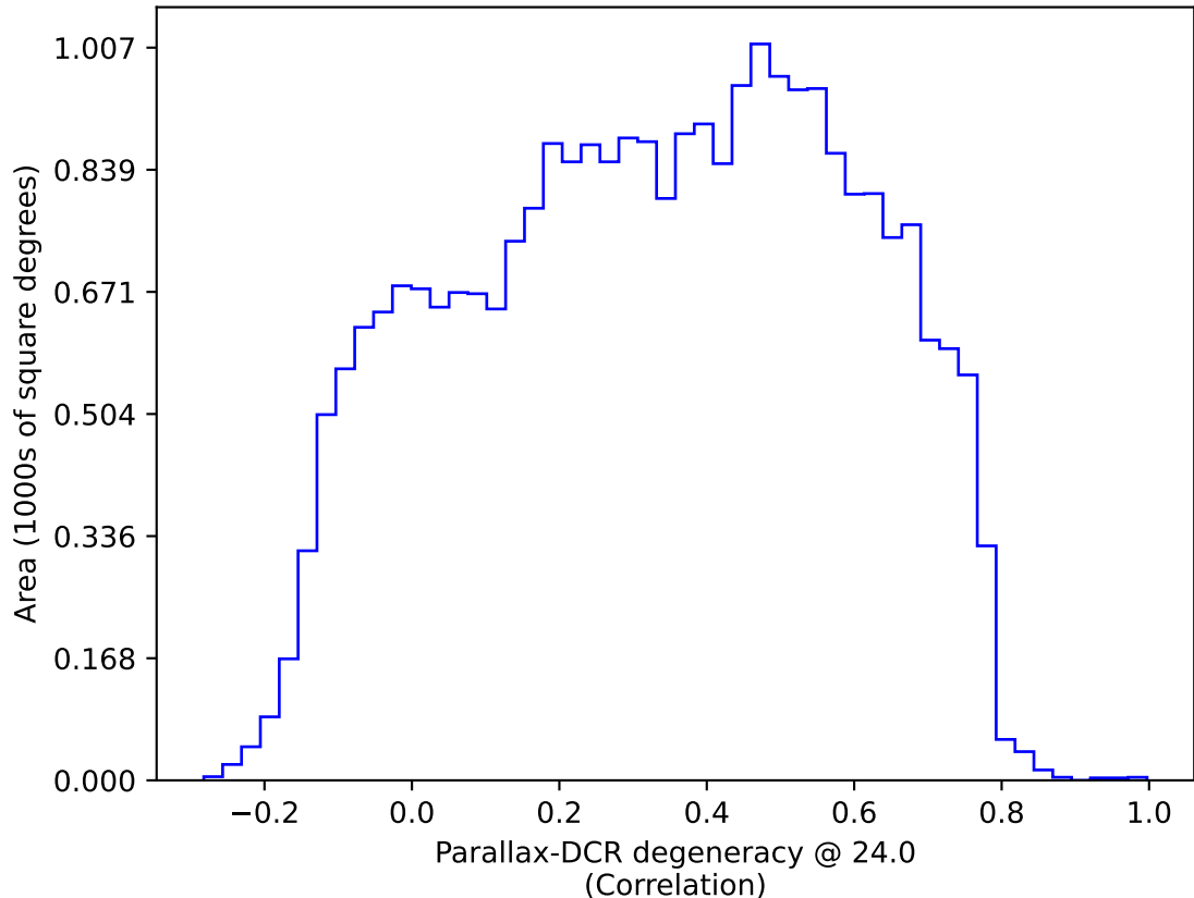
ddf_acor_sf10_ls20_lsr50_v3.4_10yrs All sky: Parallax-DCR degeneracy @ 24.0
