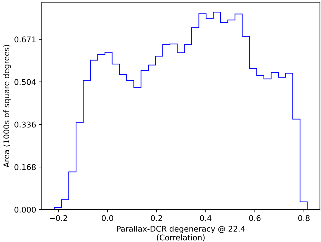
ddf_acor_sf10_lsf20_lsr50_v3.4_10yrs WFD: Parallax-DCR degeneracy @ 22.4
