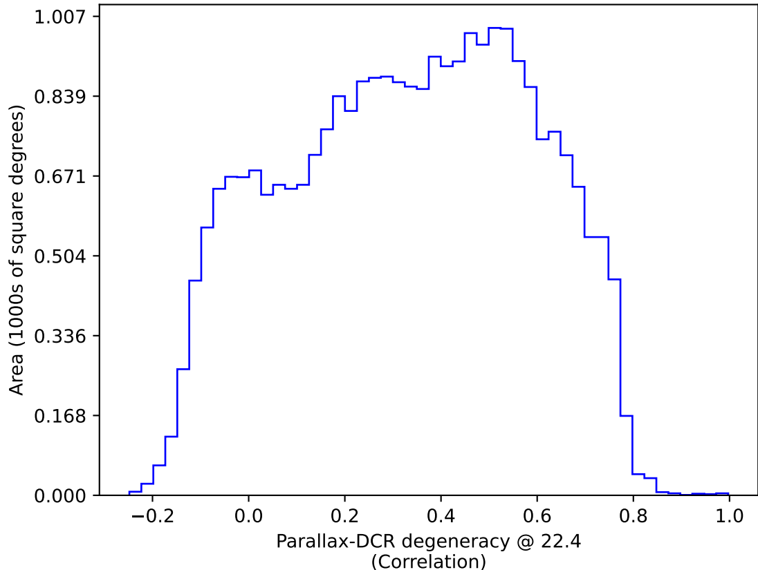
ddf_acor_sf10_ls20_lsr50_v3.4_10yrs All sky: Parallax-DCR degeneracy @ 22.4
