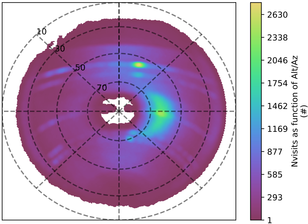
ddf_acor_sf10_lsf20_lsr50_v3.4_10yrs z band: Nvisits as function of Alt/Az
