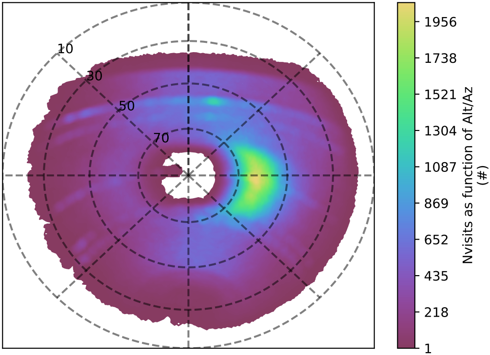
ddf_acor_sf10_lsf20_lsr50_v3.4_10yrs y band: Nvisits as function of Alt/Az
