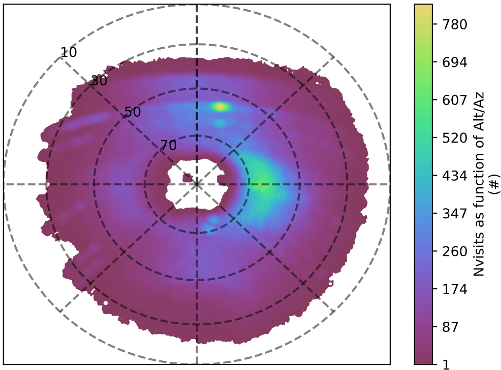
ddf_acor_sf10_lsf20_lsr50_v3.4_10yrs u band: Nvisits as function of Alt/Az
