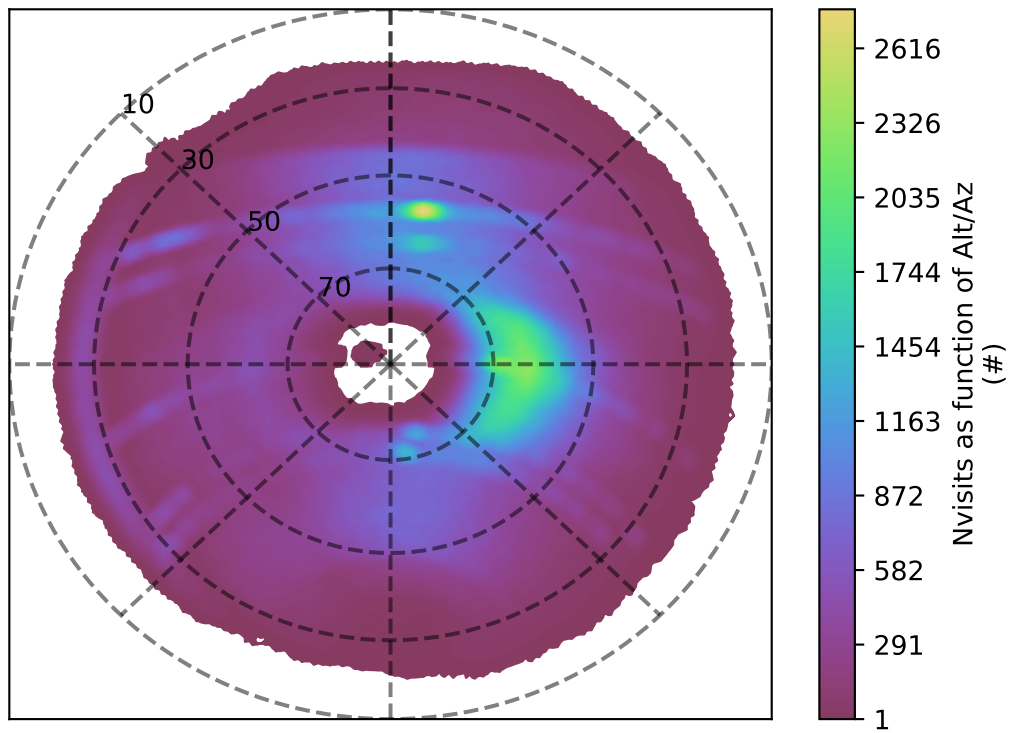
ddf_acor_sf10_lsf20_lsr50_v3.4_10yrs r band: Nvisits as function of Alt/Az
