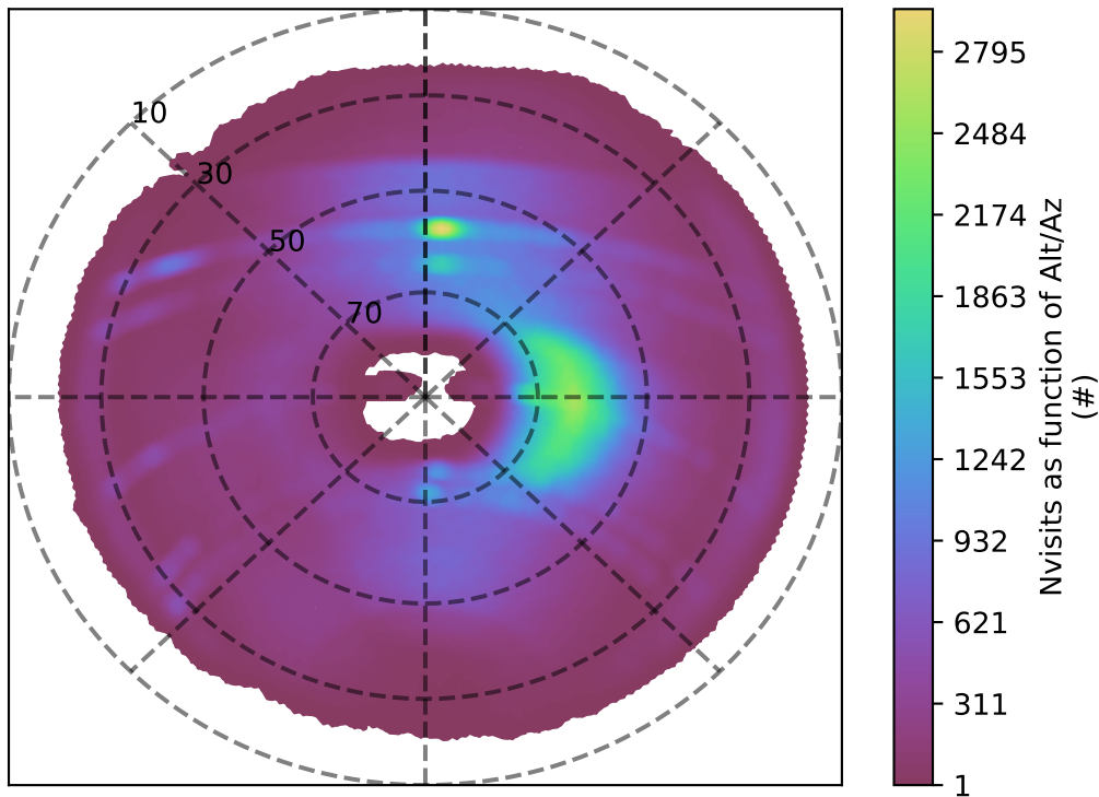
ddf_acor_sf10_lsf20_lsr50_v3.4_10yrs i band: Nvisits as function of Alt/Az
