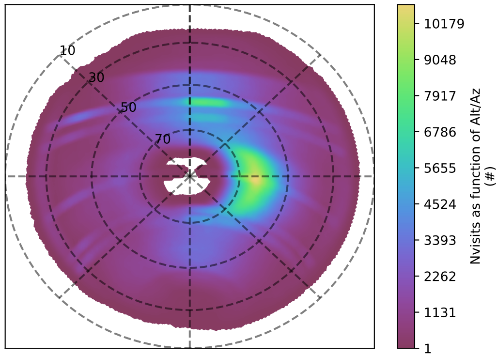
ddf_acor_sf10_ls20_lsr50_v3.4_10yrs all bands: Nvisits as function of Alt/Az
