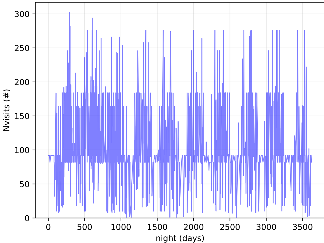
ddf_acor_sf10_lsf20_lsr50_v3.4_10yrs DDF: Nvisits
