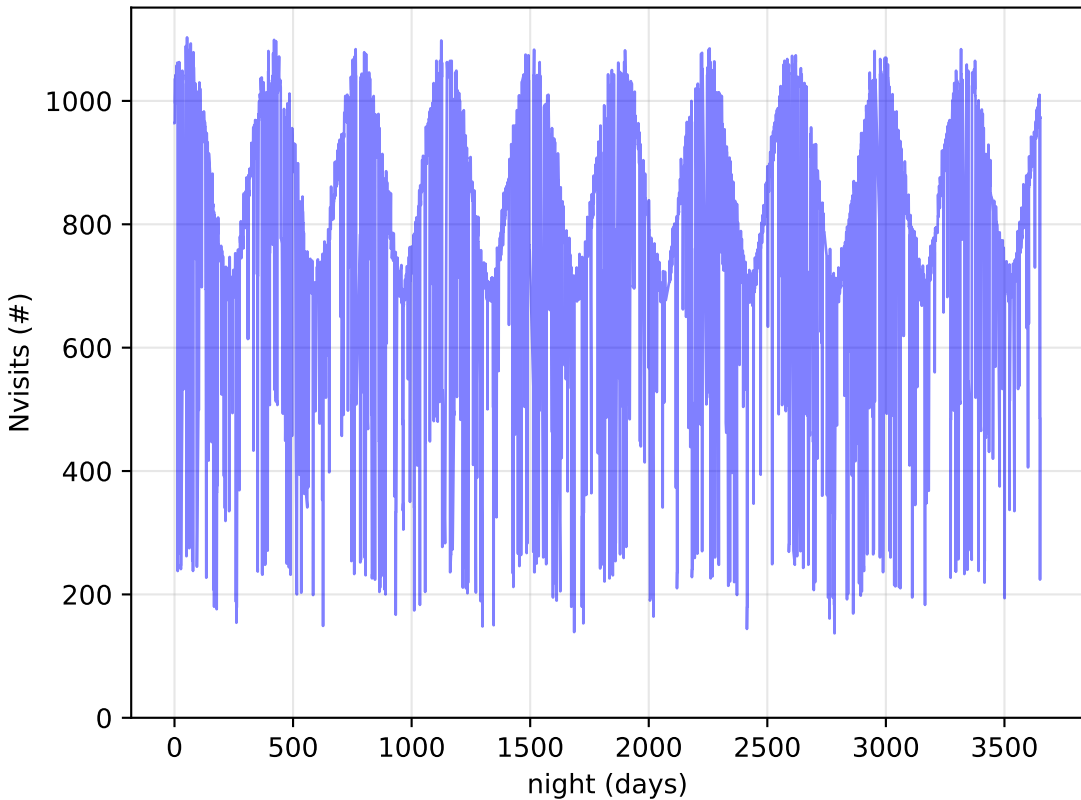
ddf_acor_sf10_ls10_lsr50_v3.4_10yrs All visits: Nvisits
