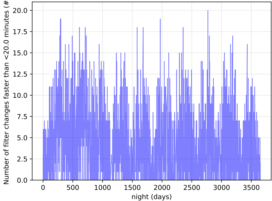
ddf_acor_sf10_Isf20_Isr50_v3.4_10yrs Per Night: Number of filter changes faster than <20.0 minutes
