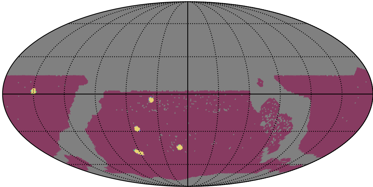
ddf_acor_sf10_lsf20_lsr50_v3.4_10yrs WFD: NumberOfQuickRevisits
