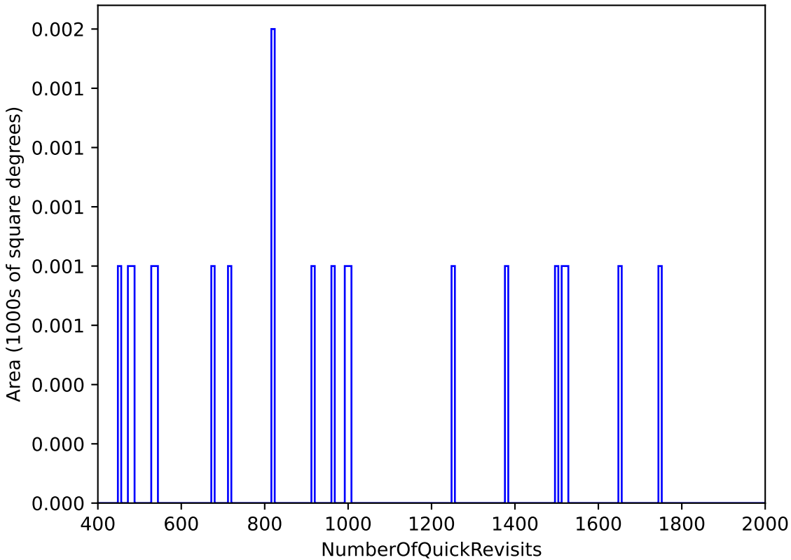
ddf_acor_sf10_lsf20_lsr50_v3.4_10yrs WFD: NumberOfQuickRevisits
