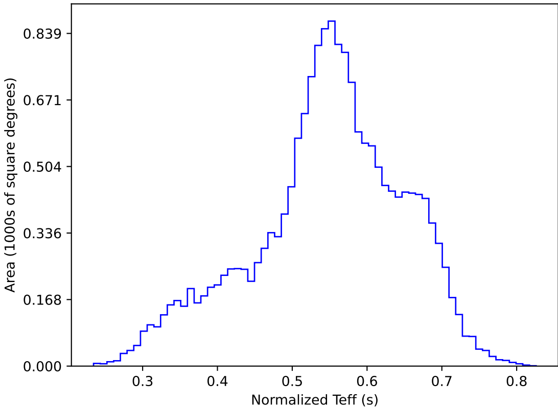
ddf_acor_sf10_lsf20_lsr50_v3.4_10yrs WFD y band: Normalized Teff
