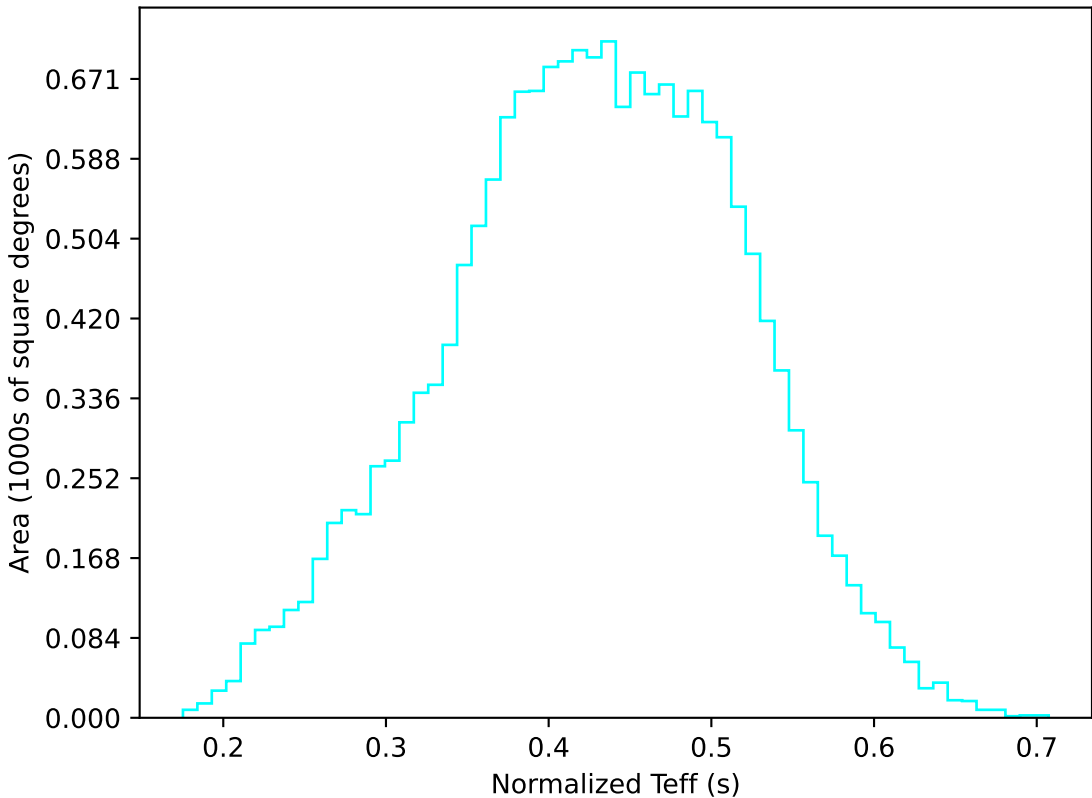
ddf_acor_sf10_lsf20_lsr50_v3.4_10yrs WFD u band: Normalized Teff
