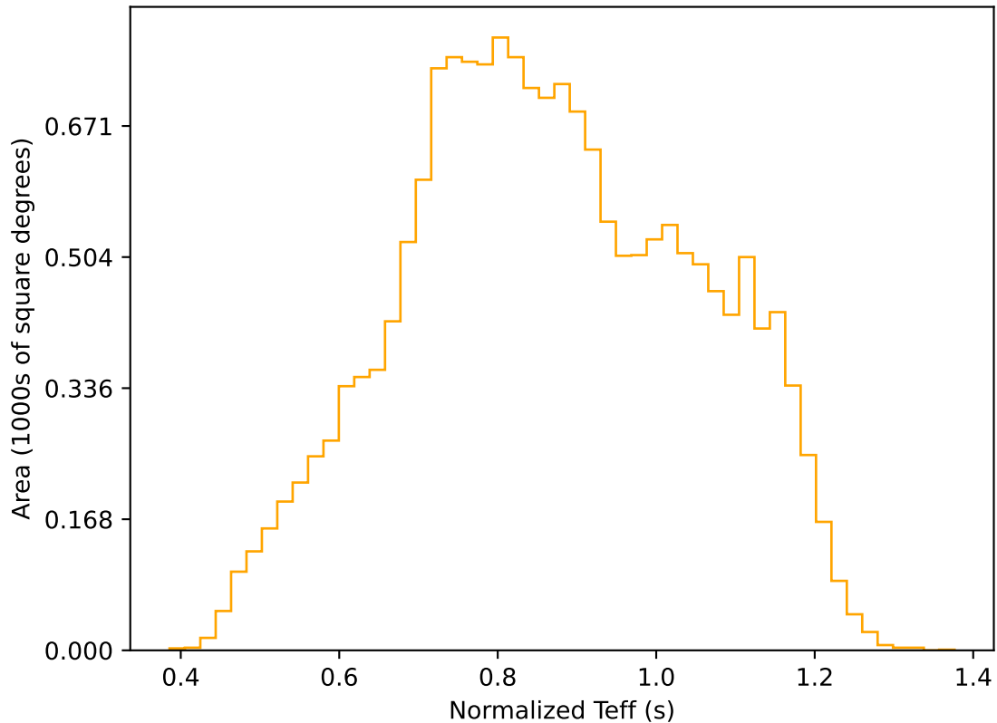
ddf_acor_sf10_lsf20_lsr50_v3.4_10yrs WFD r band: Normalized Teff
