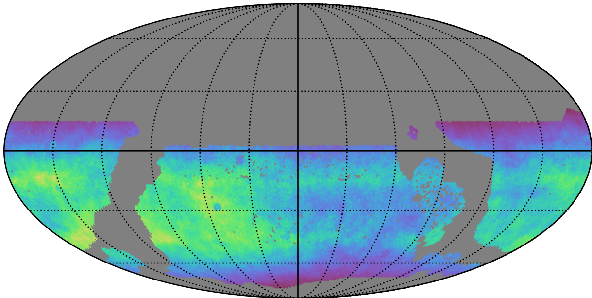
ddf_acor_sf10_lsf20_lsr50_v3.4_10yrs WFD i band: Normalized Teff
