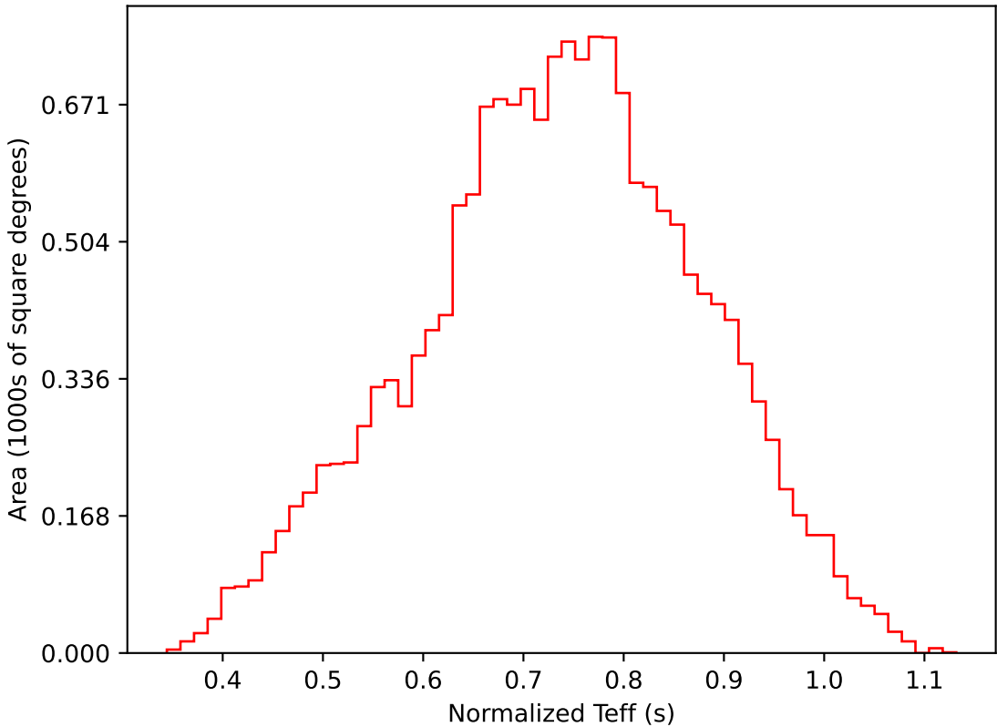
ddf_acor_sf10_lsf20_lsr50_v3.4_10yrs WFD i band: Normalized Teff
