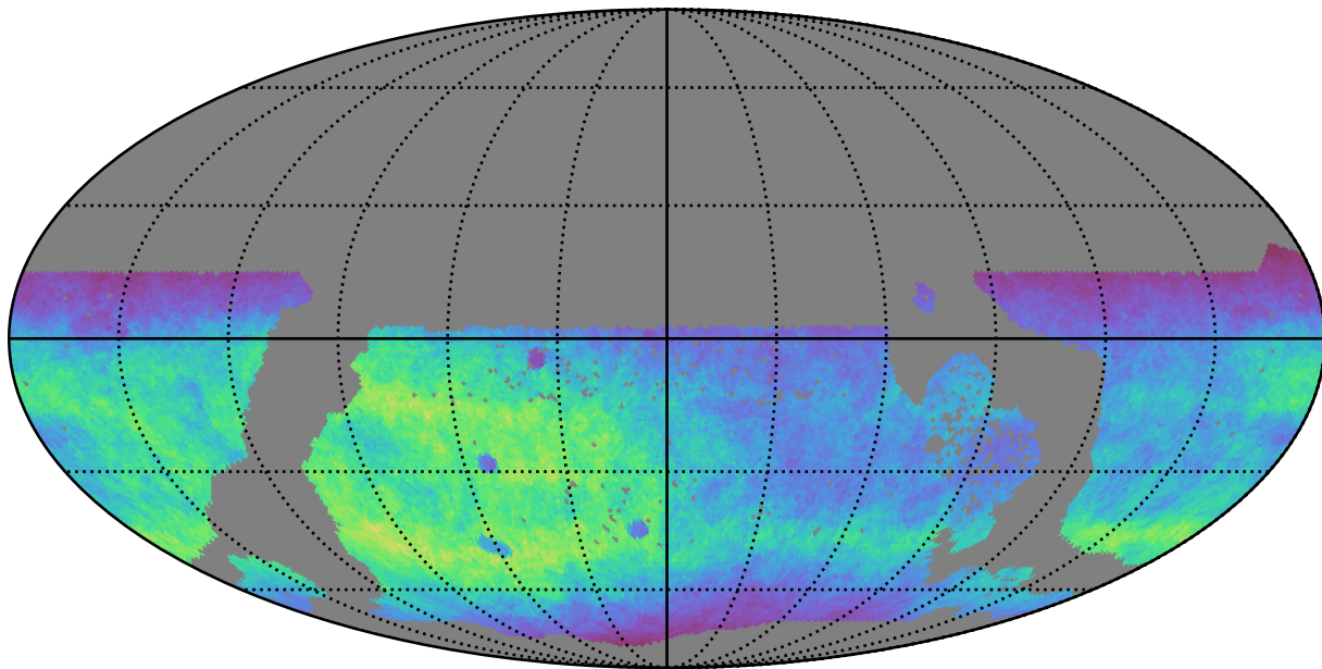
ddf_acor_sf10_lsf20_lsr50_v3.4_10yrs WFD g band: Normalized Teff
