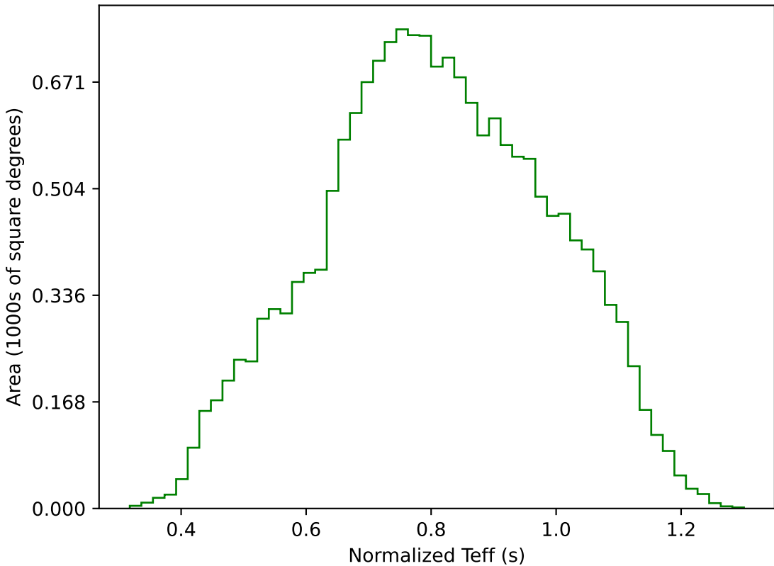
ddf_acor_sf10_lsf20_lsr50_v3.4_10yrs WFD g band: Normalized Teff
