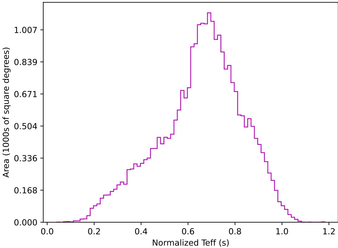
ddf_acor_sf10_lsf20_lsr50_v3.4_10yrs All sky z band: Normalized Teff
