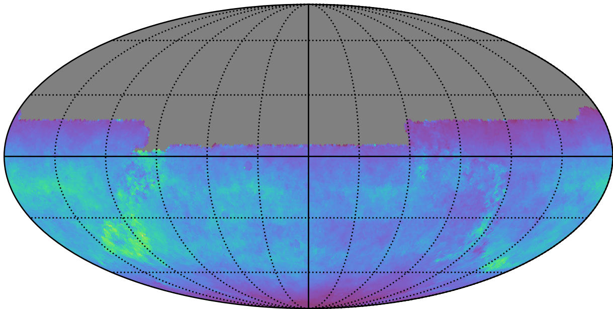
ddf_acor_sf10_lsf20_lsr50_v3.4_10yrs All sky u band: Normalized Teff
