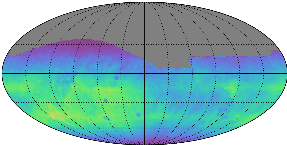
ddf_acor_sf10_lsf20_lsr50_v3.4_10yrs All sky r band: Normalized Teff
