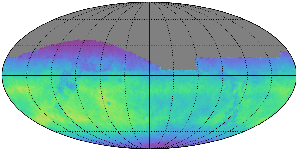
ddf_acor_sf10_lsf20_lsr50_v3.4_10yrs All sky i band: Normalized Teff
