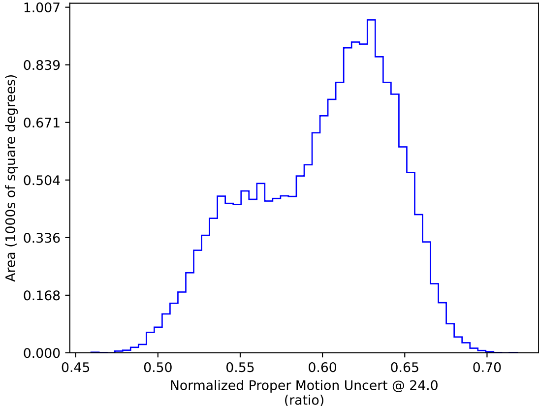
ddf_acor_sf10_lsf20_lsr50_v3.4_10yrs WFD: Normalized Proper Motion Uncert @ 24.0
