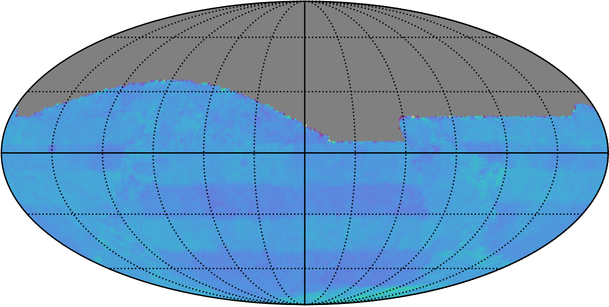
ddf_acor_sf10_lsf20_lsr50_v3.4_10yrs All sky: Normalized Proper Motion Uncert @ 24.0
