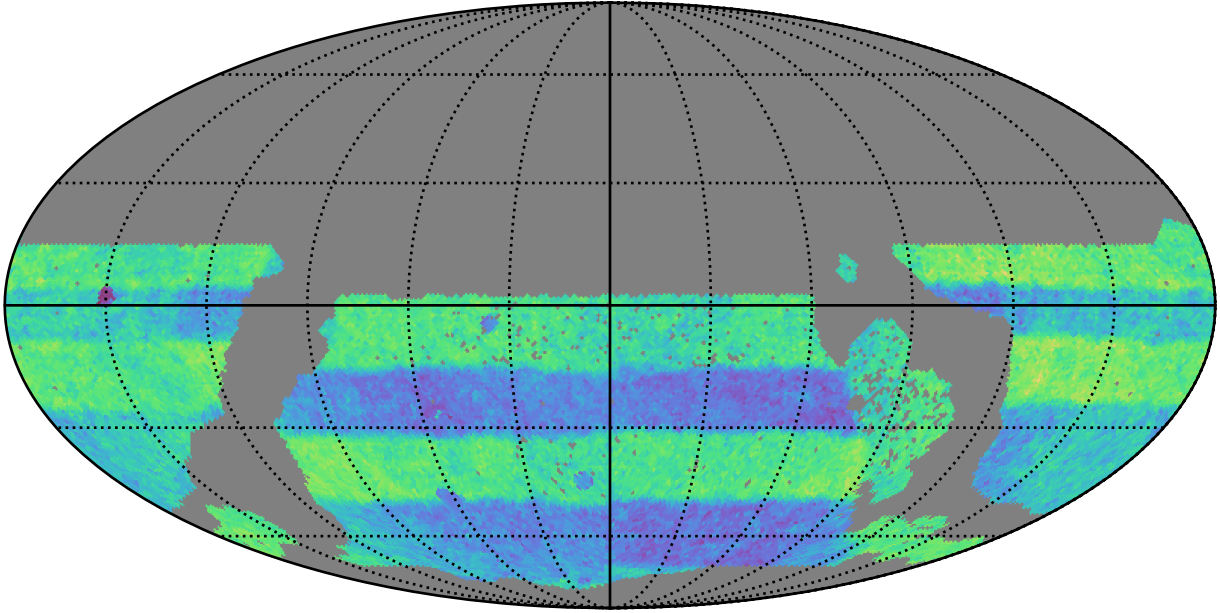
ddf_acor_sf10_lsf20_lsr50_v3.4_10yrs WFD: Normalized Proper Motion Uncert @ 20.5
