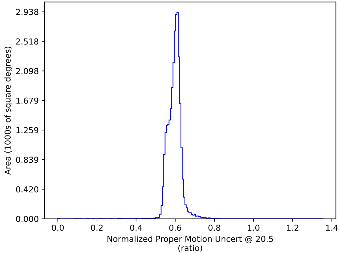
ddf_acor_sf10_lsf20_lsr50_v3.4_10yrs All sky: Normalized Proper Motion Uncert @ 20.5
