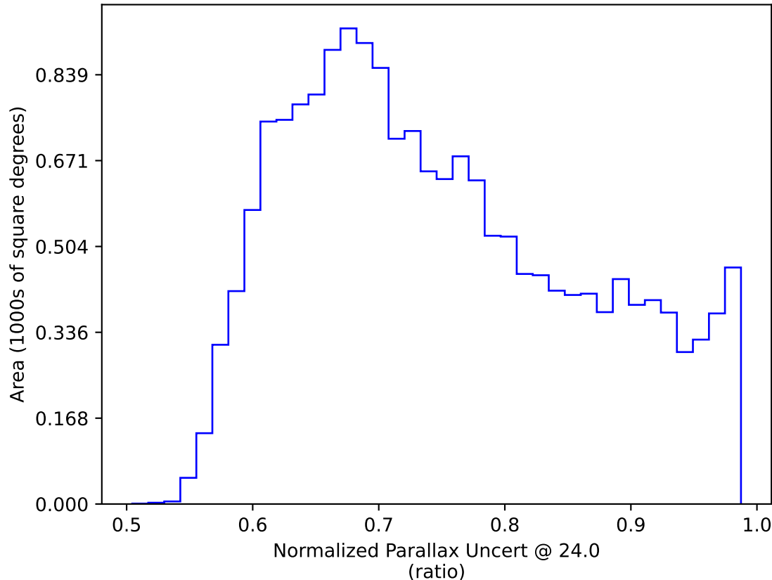
ddf_acor_sf10_lsf20_lsr50_v3.4_10yrs WFD: Normalized Parallax Uncert @ 24.0
