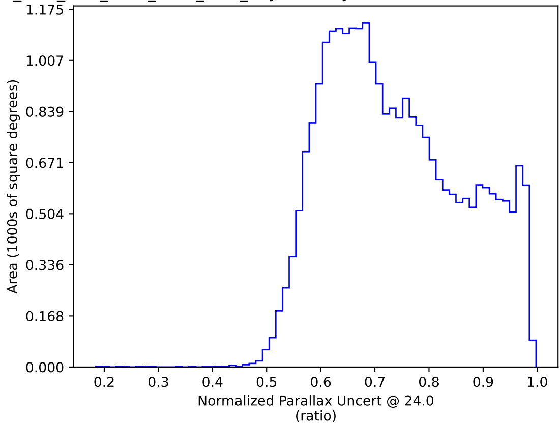
ddf_acor_sf10_lsf20_lsr50_v3.4_10yrs All sky: Normalized Parallax Uncert @ 24.0
