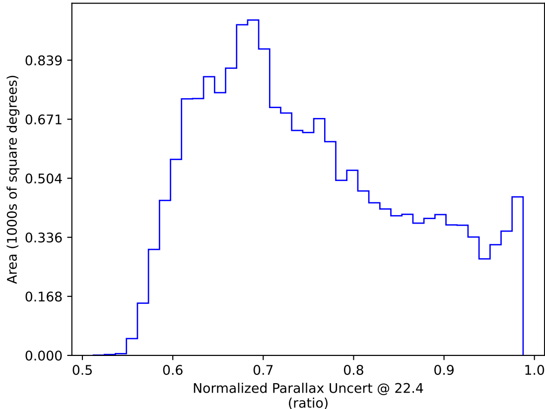
ddf_acor_sf10_lsf20_lsr50_v3.4_10yrs WFD: Normalized Parallax Uncert @ 22.4
