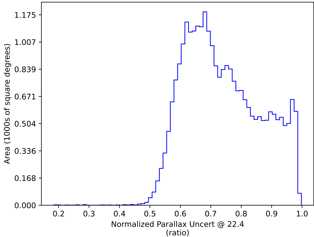
ddf_acor_sf10_lsf20_lsr50_v3.4_10yrs All sky: Normalized Parallax Uncert @ 22.4
