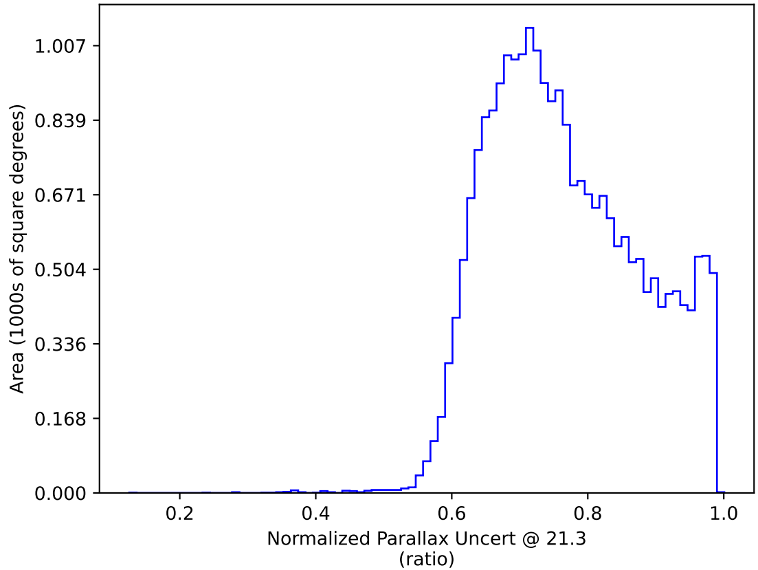
ddf_acor_sf10_lsf20_lsr50_v3.4_10yrs All sky y band only: Normalized Parallax Uncert @ 21.3
