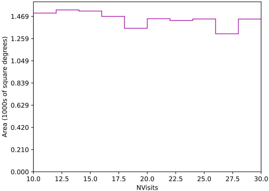
ddf_acor_sf10_lsf20_lsr50_v3.4_10yrs Yr 3-4 z band: NVisits
