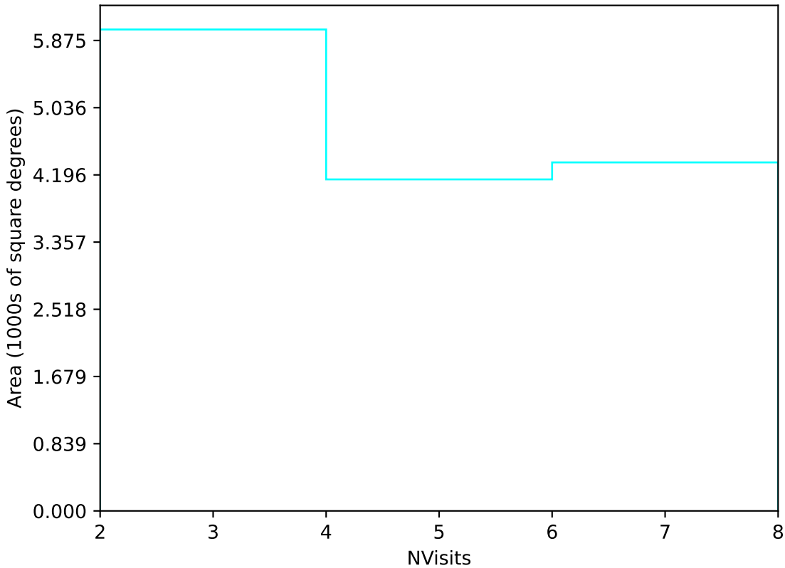
ddf_acor_sf10_lsf20_lsr50_v3.4_10yrs Yr 3-4 u band: NVisits
