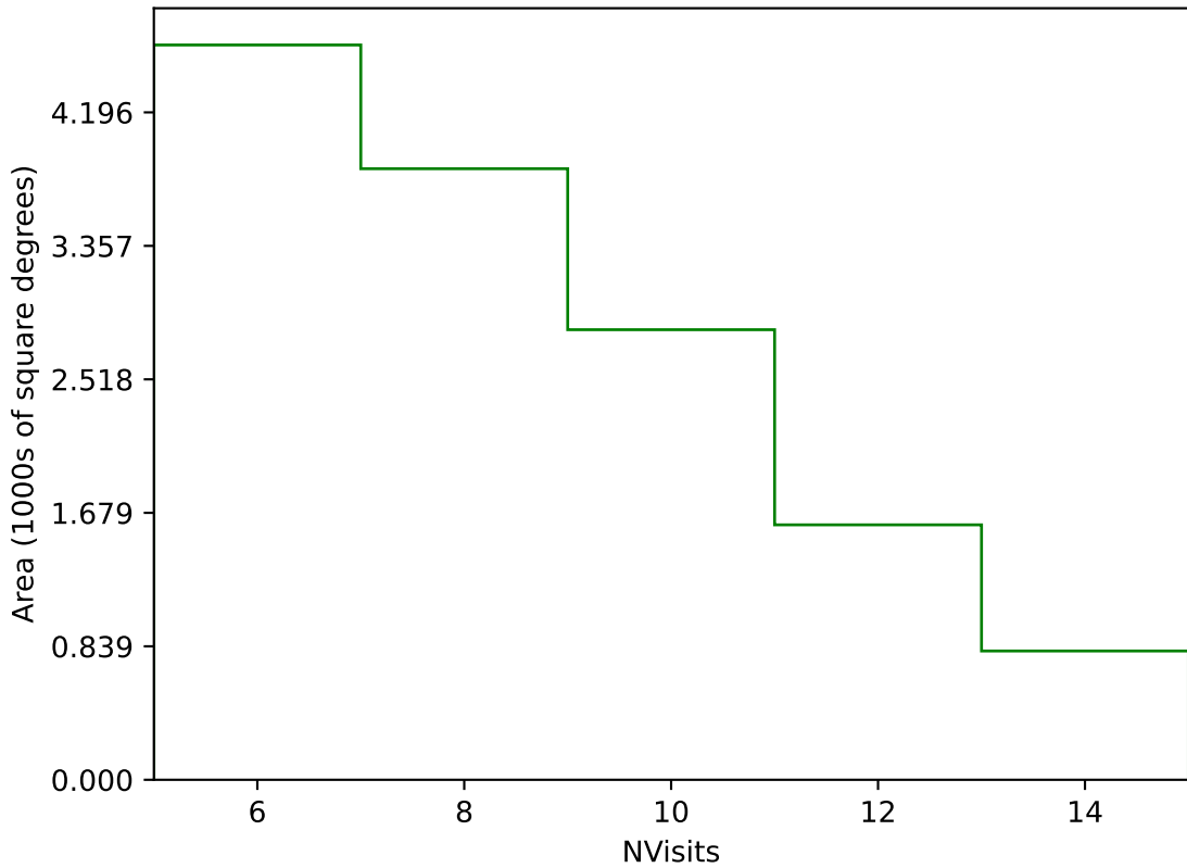
ddf_acor_sf10_lsf20_lsr50_v3.4_10yrs Yr 3-4 g band: NVisits
