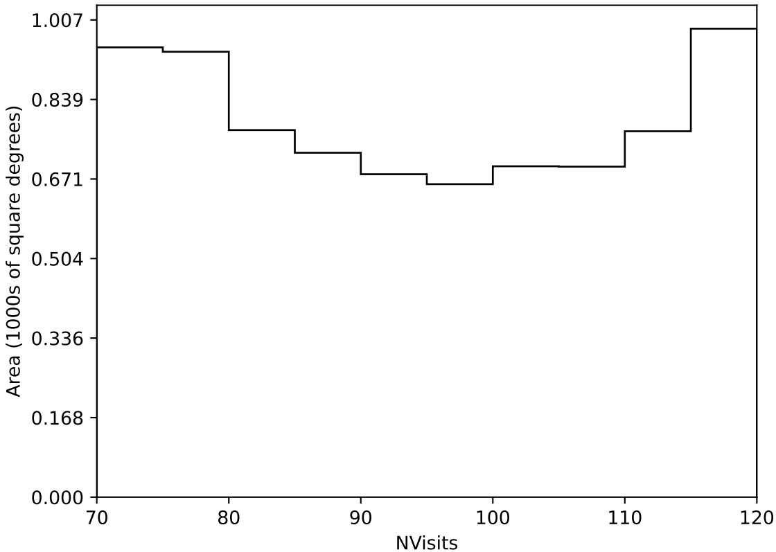
ddf_acor_sf10_lsf20_lsr50_v3.4_10yrs Yr 3-4 all bands: NVisits
