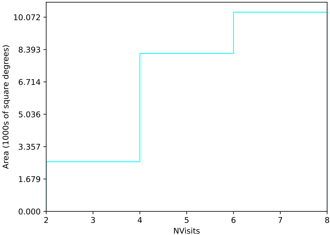
ddf_acor_sf10_lsf20_lsr50_v3.4_10yrs Yr 1 u band: NVisits
