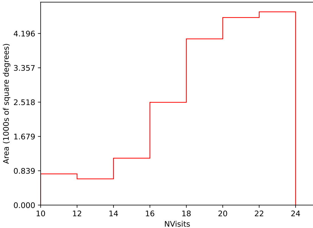
ddf_acor_sf10_lsf20_lsr50_v3.4_10yrs Yr 1 i band: NVisits
