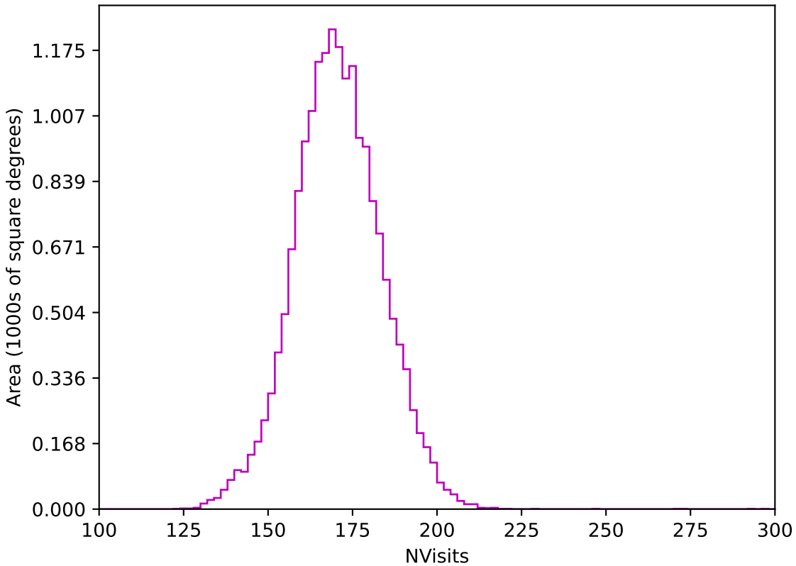
ddf_acor_sf10_lsf20_lsr50_v3.4_10yrs WFD z band: NVisits
