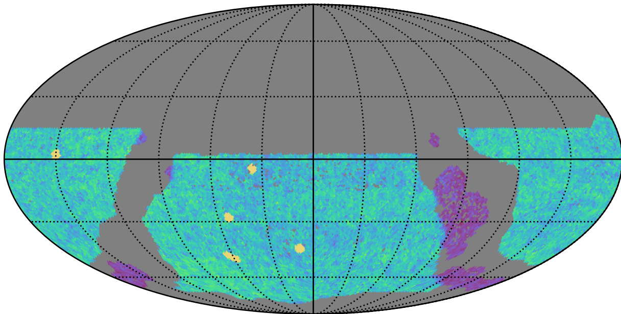
ddf_acor_sf10_lsf20_lsr50_v3.4_10yrs WFD u band: NVisits
