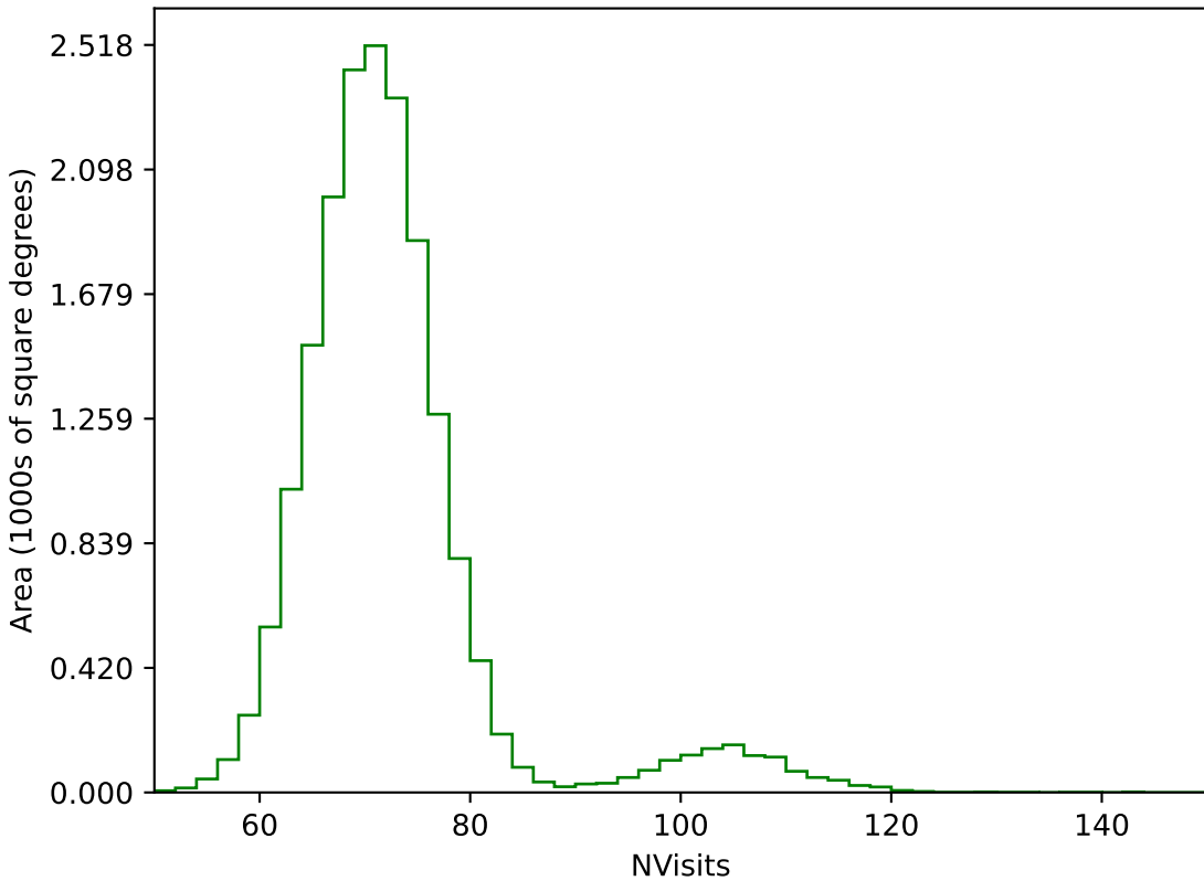
ddf_acor_sf10_lsf20_lsr50_v3.4_10yrs WFD g band: NVisits
