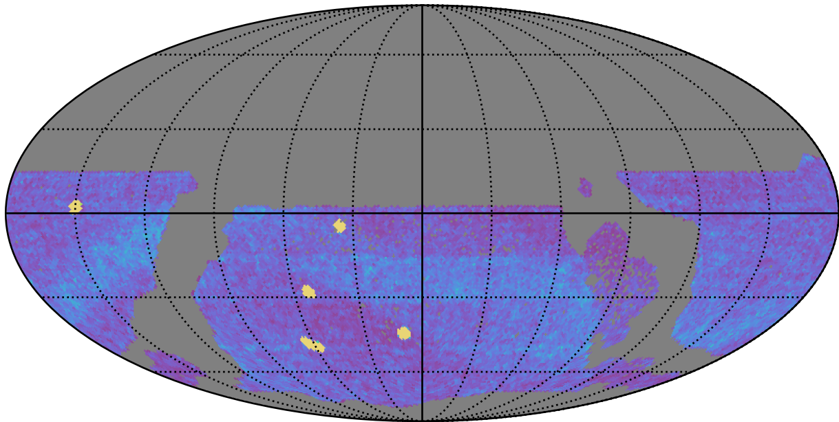
ddf_acor_sf10_lsf20_lsr50_v3.4_10yrs WFD all bands: NVisits
