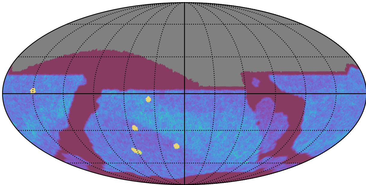
ddf_acor_sf10_lsf20_lsr50_v3.4_10yrs All sky z band: NVisits
