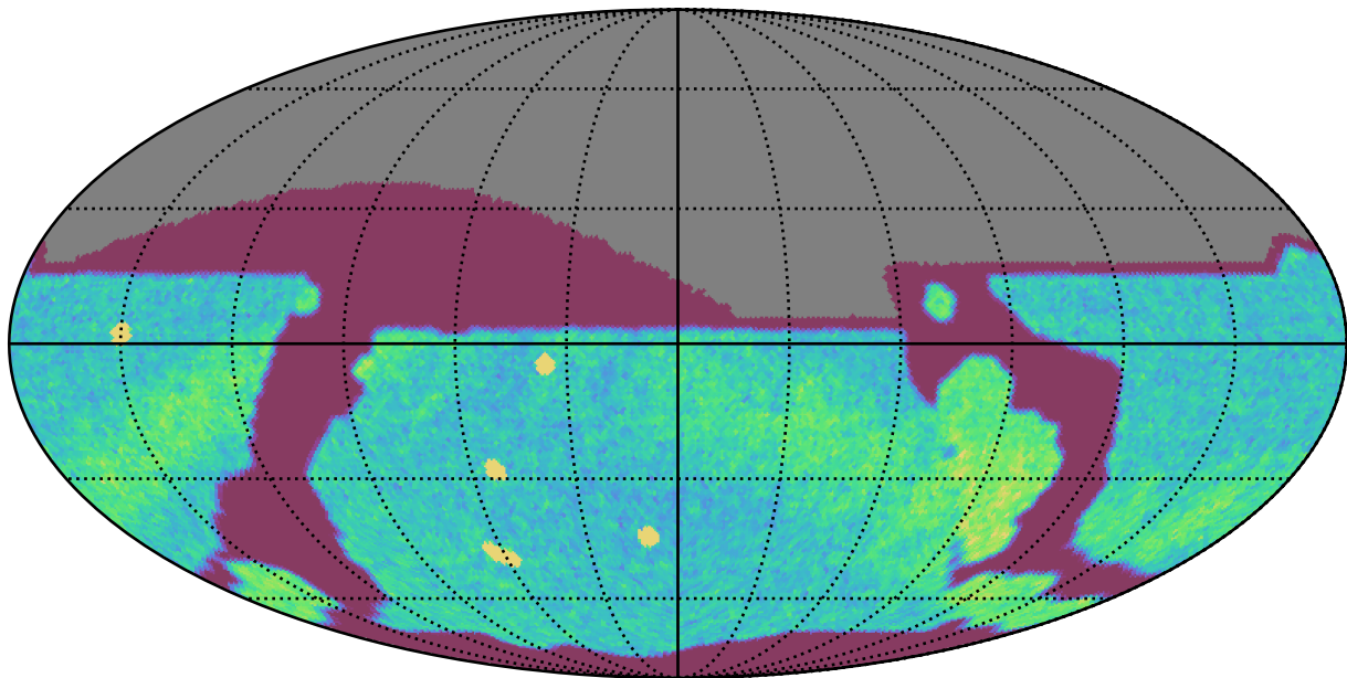
ddf_acor_sf10_lsf20_lsr50_v3.4_10yrs All sky r band: NVisits
