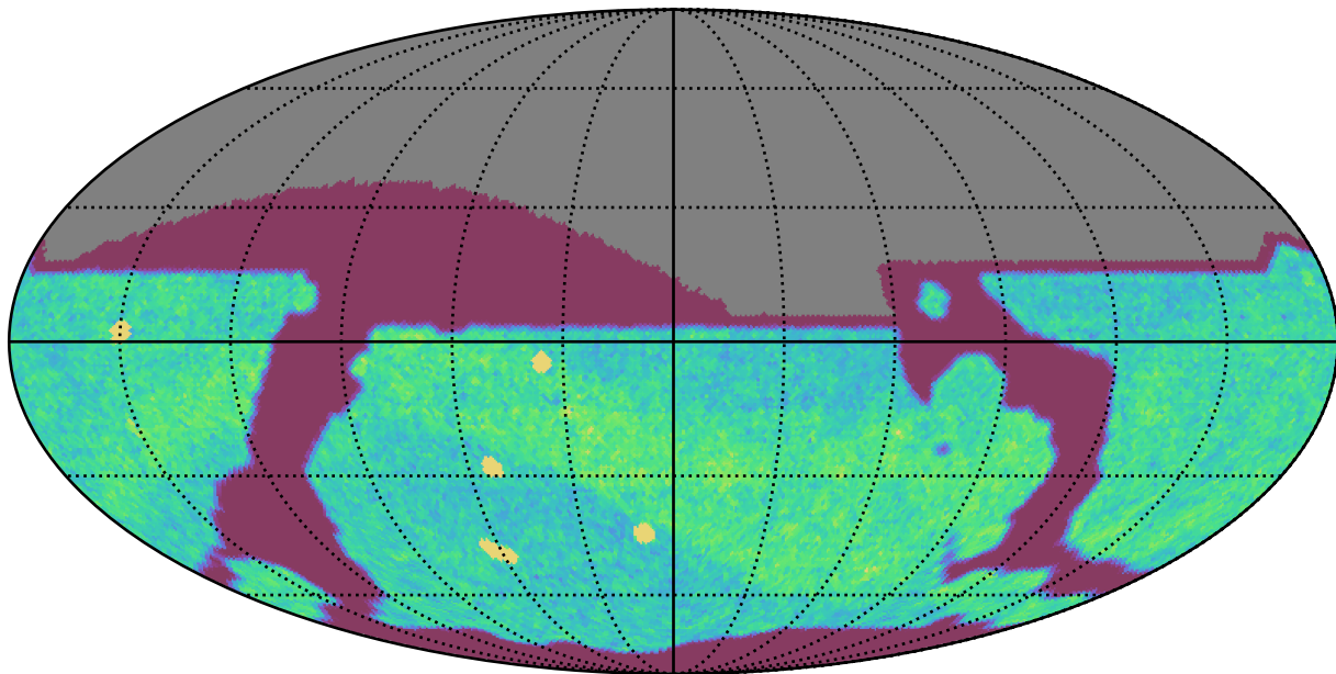
ddf_acor_sf10_lsf20_lsr50_v3.4_10yrs All sky i band: NVisits
